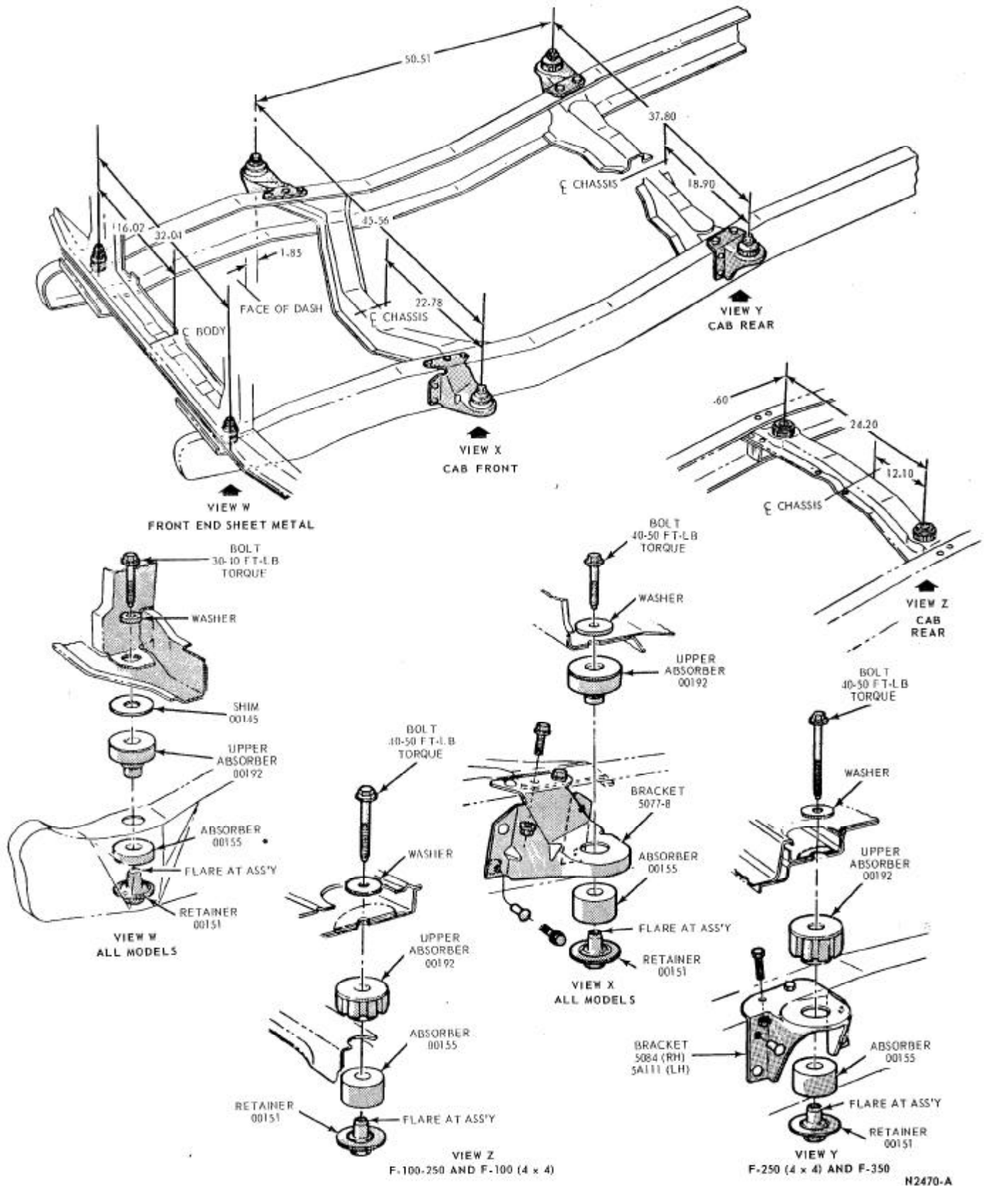
FIG. 7 Body Mounts
