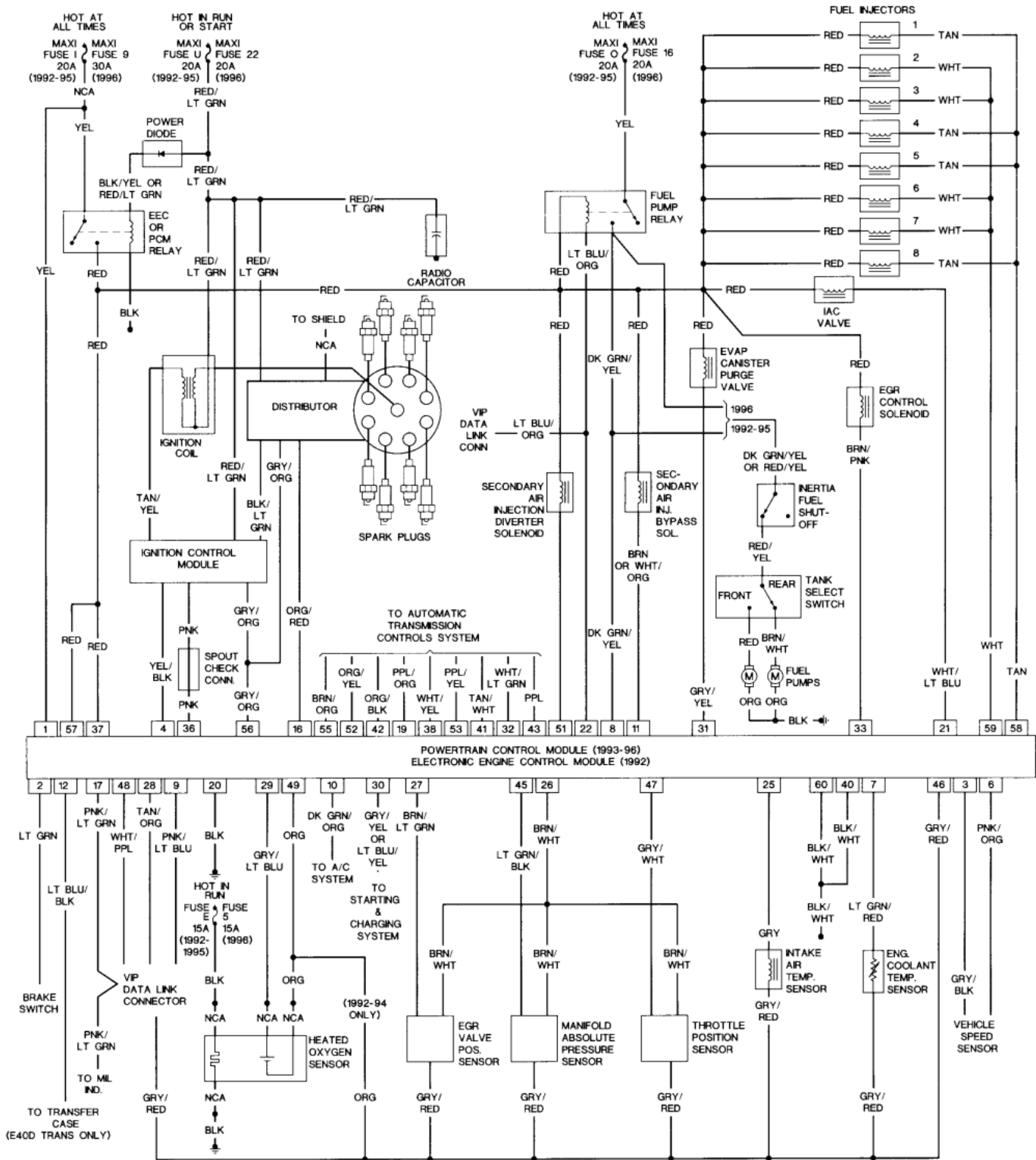
FIG : Fig. 22: Engine wiring-1992-95 F-Series 7.5L (VIN G), 1996 F-Series 7.5L Federal (VIN G) and 1996 F-Series Pick-up 5.8L (VIN H over 8500 GVW) engines
